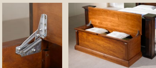
Ref. 5035 - Baú L 138 x A 55 x P 44
